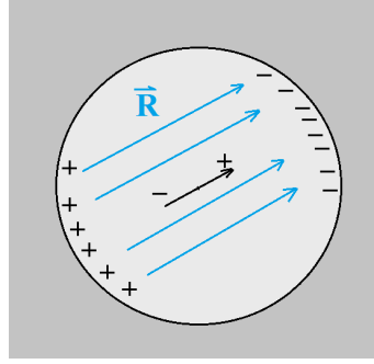
Figure 2.1: Illustration of the reaction field around a molecular dipole.
