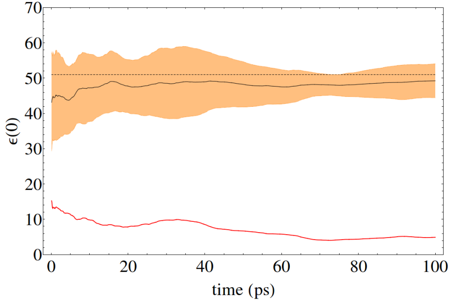
Figure 4.9: Running average of \epsilon(0) at 330 K over ten runs calculated from the Kirkwood G-factor found using the integration method ( eqn. 6.20).
