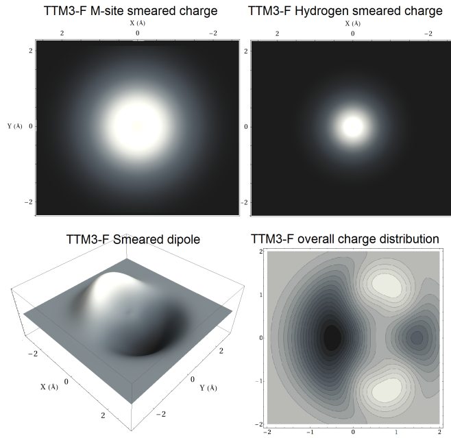
Figure 4.1: Smeared charges, smeared dipole and the total equilibrium charge distribution.
