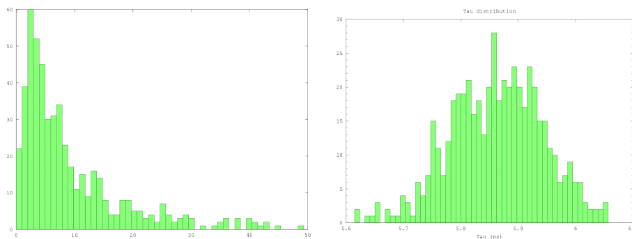
Figure 8.8: Distribution of \tau when the correlation function for each molecule is analyzed separately for 512 TIP4P/2005 at 300 K for 10 ps (left) and 2ns (right).
