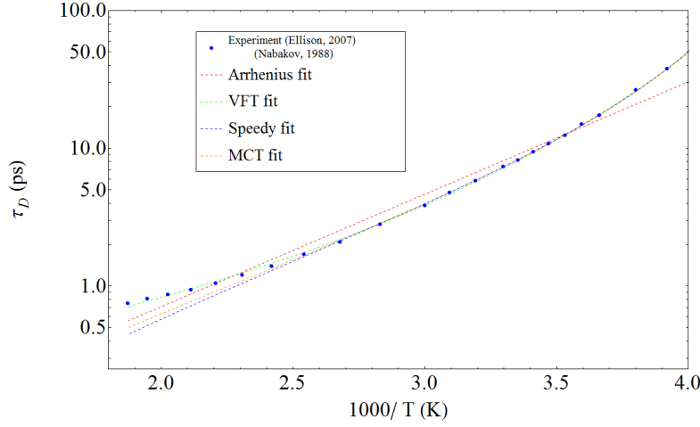
Figure 8.2: Arrhenius plot of \tau_D(T) from experimental data, [103, 283] showing several fit functions. Only the VFT relaxation equation is capable of reproducing the experimental data over the full temperature range.
