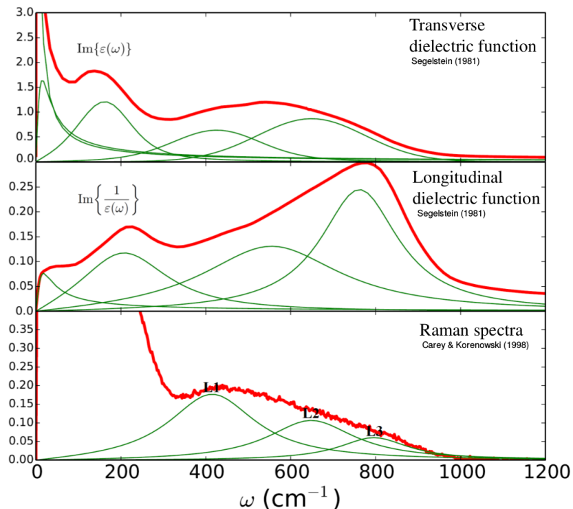
Figure 10.2: A figure highlighting the discrepancy in peak assignment. Dielectric functions derived from a compilation of experimental data by Segelstein,[367] with fits by D. C. Elton, while the Raman data comes from (Carey, 1998).[65] The Raman peaks are not fit but merely placed at the positions reported from Carey’s fit.
