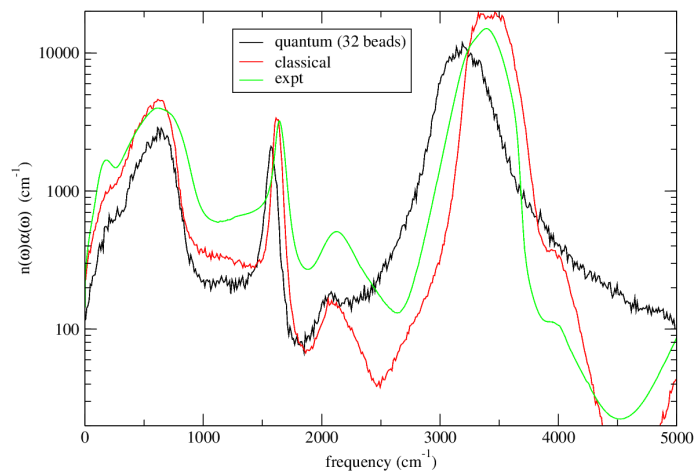
Figure 11.7: Infrared spectra for TTM3F at 300 K, plotted on a log scale to show detail. Experimental data from Bertie & Lan, 1996.[38] PA-CMD was used, with normal mode frequencies scaled to 5000 \text{ cm}^{-1} .
