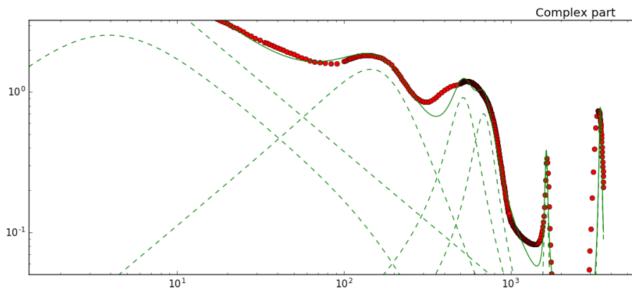
Figure 7.2: Example of fitting the imaginary part of the dielectric function from Segelstein's collection of experimental data.[367] NOTE: this will be replaced with a much better figure / fit
