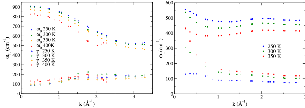
Figure 10.13: Longitudinal (left) and transverse (right) dispersion relations (circles) and dampening factors (squares) for 512 TIP4P/2005f. These curves were obtained from a two peak (Debye + resonant) fit. In contrast to the longitudinal mode, the transverse mode is much more damped.
