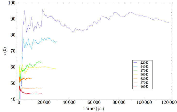
Figure 4.4: Convergence of \epsilon(0) for 512 TIP4P/2005.
