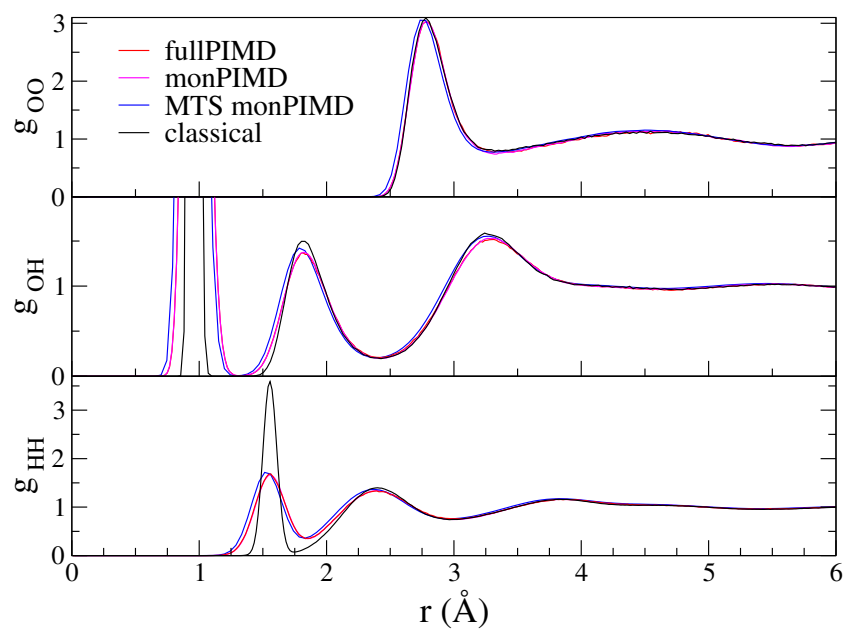
Figure 12.2: Validation with TTM3F: RDFs for the three methods at 300 K.
