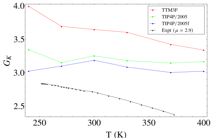
Figure 5.5: G_K(r) for the models at different temperatures, calculated using \varepsilon(0)(T) and \mu(T) . The experimental data was calculated using experimental \varepsilon(0) [119, 40] using eqn. 4.23 and \mu = 2.9 .
