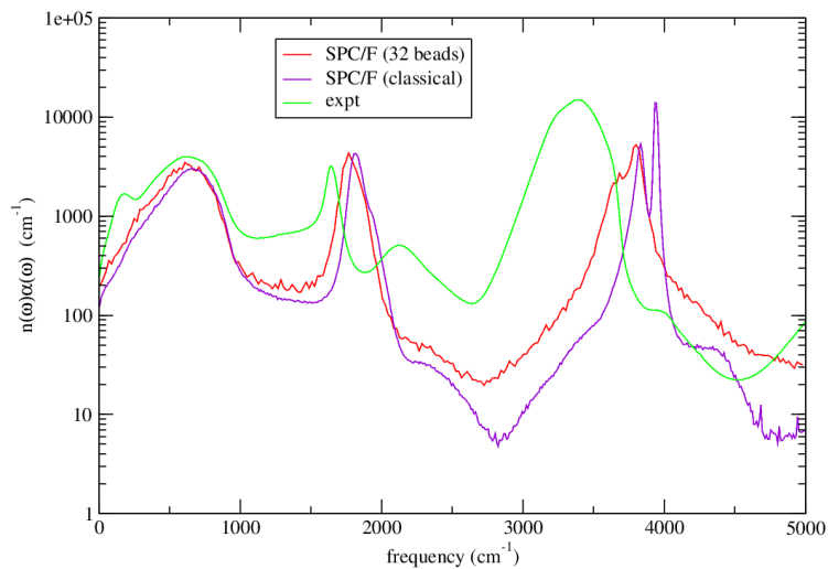
Figure 11.8: Infrared spectra for SPC/F at 300 K. Experimental data from Bertie & Lan, 1996.[38] PA-CMD was used, with normal mode frequencies scaled to 5000 \text{ cm}^{-1} .
