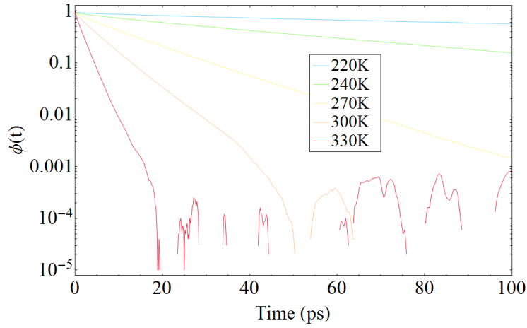
Figure 8.7: Single molecule correlation functions for TIP4P/2005.
