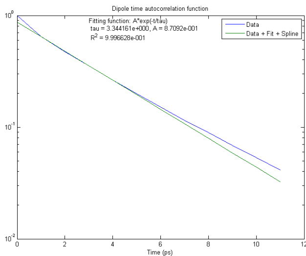
Figure 8.6: An example fit of the single molecule correlation function for TTM3F at 300 K.
