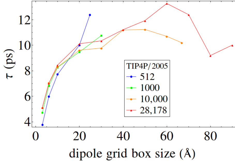
Figure 7.3: Debye relaxation calculated with different box sizes. This clearly shows that Debye relaxation is a collective phenomena, requiring box sizes of \approx 2\text{nm} for convergence.
