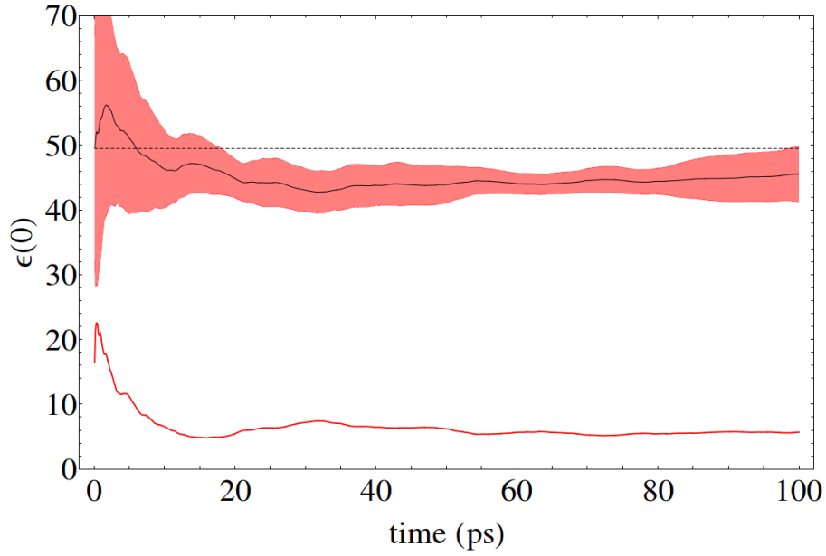
Figure 4.10: Running average of \epsilon(0) at 370 K over ten runs calculated from the Kirkwood G-factor found using the integration method ( eqn. 6.20).
