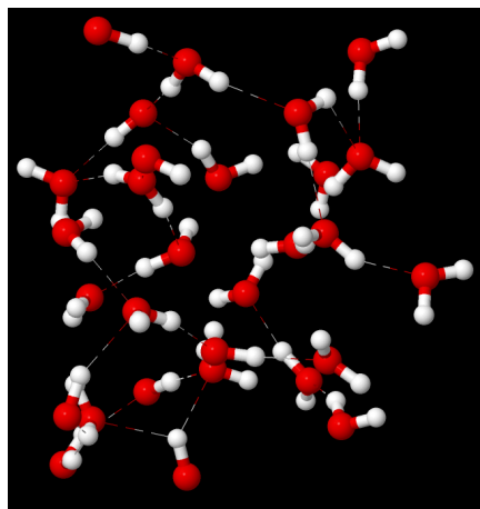
Figure 1.3: Schematic cross section of water, showing the H-bond network.
