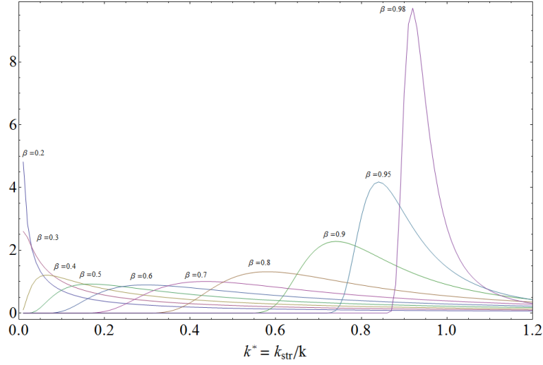
Figure 8.4: G(k) distribution for various values of \beta .
