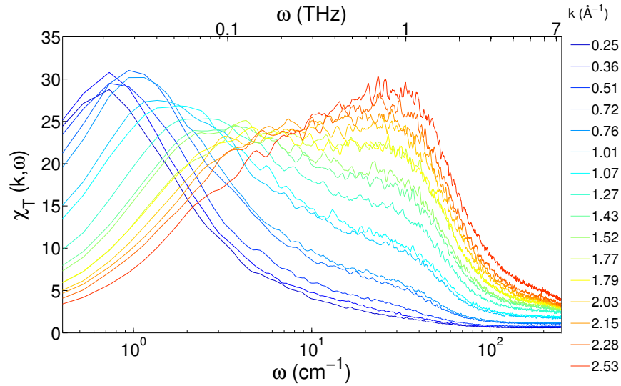
Figure 7.4: k dependence of the Debye relaxation (left most peak) for TIP4P/2005f.
