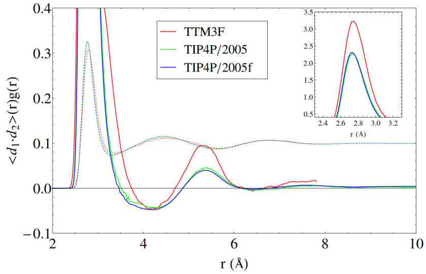
Figure 6.8: The dip-dip correlation function defined by equation 6.5. The O-O RDFs (rescaled by a factor of .1) are shown for comparison.
