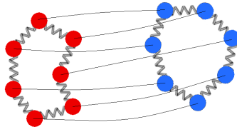
Figure 11.2: Illustration of the interaction of two atoms in PIMD, each represented by ring polymers.
