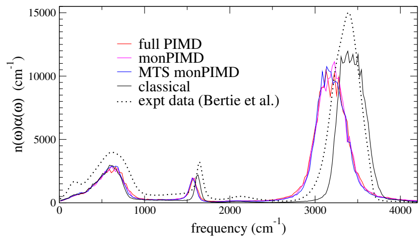
Figure 12.3: Validation with TTM3F: infrared spectra for the three PIMD methods compared to the classical spectra and experimental data at 300 K. [38]
