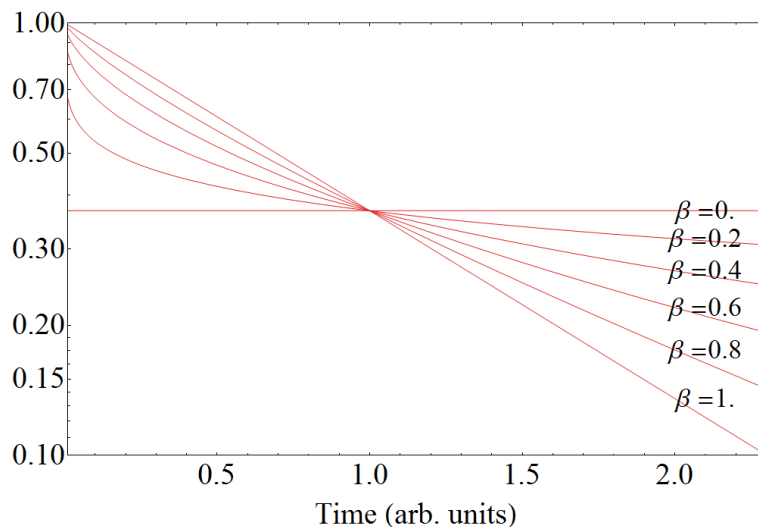
Figure 8.3: The stretched exponential function for various values of \beta .
