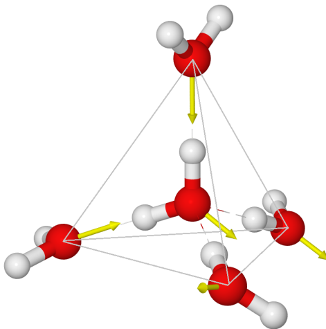
Figure 1.1: Schematic of the tetrahedral coordination of water. The yellow arrows show dipole moment. Overall, the 5 molecule tetrahedron has a larger dipole than that of a single molecule.
