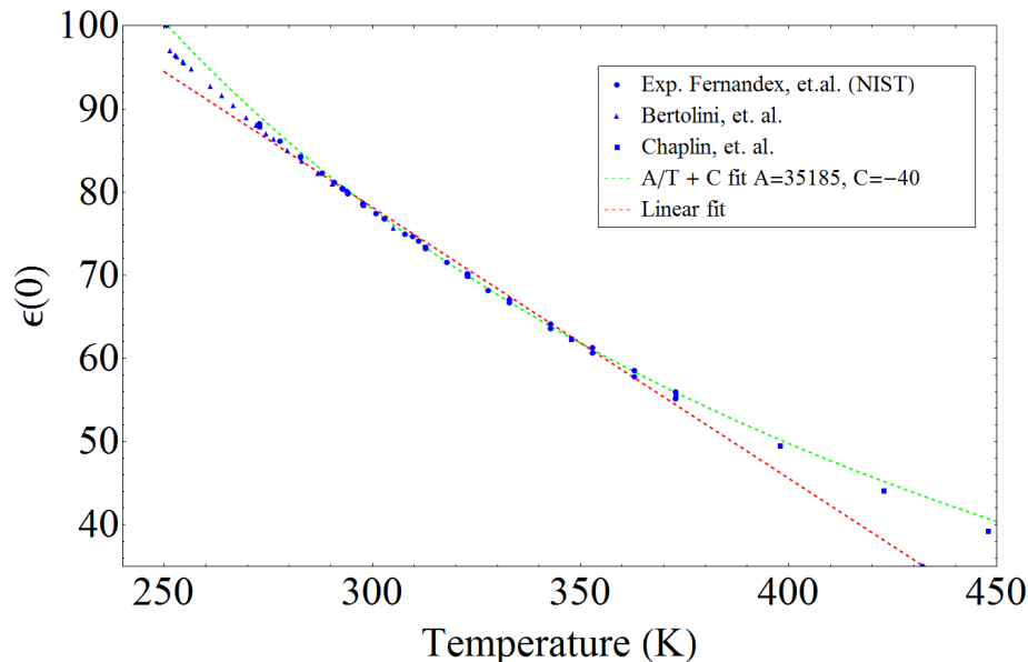
Figure 1.2: Experimental data on \epsilon(0) . Although a \epsilon(0)(T) is roughly linear in the range 273 - 373 K, the overall behaviour is better described by A/T + C . The data above 373 K is taken along the liquid-vapor coexistence curve with increased pressure.
