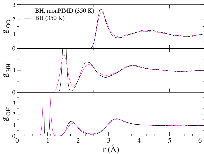
Figure 12.8: Comparison of BH simulated with the monomer PIMD method (with the monomer correction) compared to a conventional BH simulation. The simulation was performed at 350 K here to compare with PBE at the same temperature.
