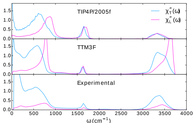
Figure 10.14: Imaginary parts of the static transverse and longitudinal dielectric susceptibility for TIP4P/2005f, TTM3F, and experimental data[11] at 298 K. The effects of polarization can be seen in the LO-TO splitting of the stretching mode and in the low frequency features.
