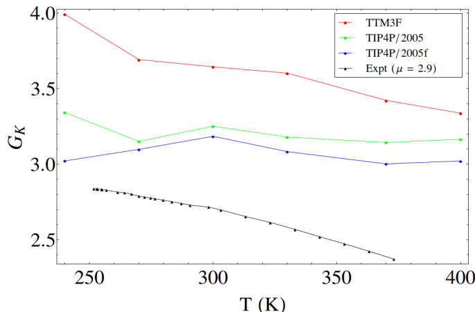
Figure 5.5: G_K(r) for the models at different temperatures, calculated using \epsilon(0)(T) and \mu(T) . The experimental data was calculated using experimental \epsilon(0) [1, 2] using eqn. 4.23 and \mu = 2.9 .
