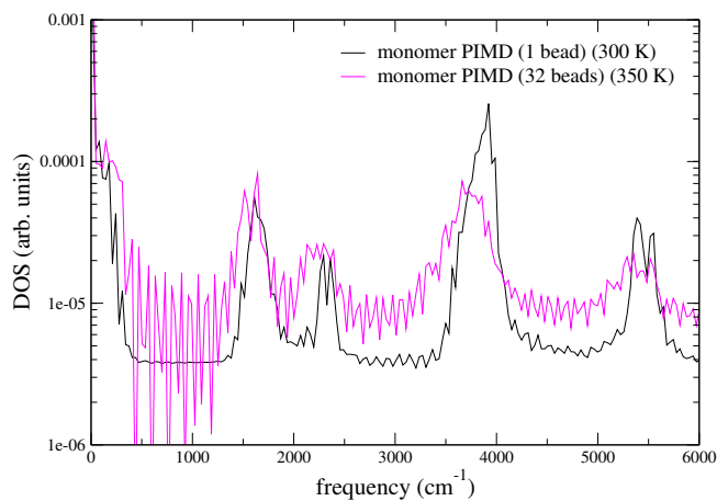
Figure 12.6: Density of states (eqn. 12.27) for a single molecule simulated with the monomer PIMD method with 1 bead and 32 beads. The monomer PIMD simulation exhibits extra peaks at \approx 2250 \text{ cm}^{-1} and \approx 5250 \text{ cm}^{-1} .
