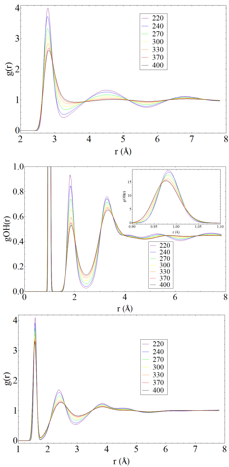
Figure A.2: RDFs at different temperatures for 128 TTM3F.
