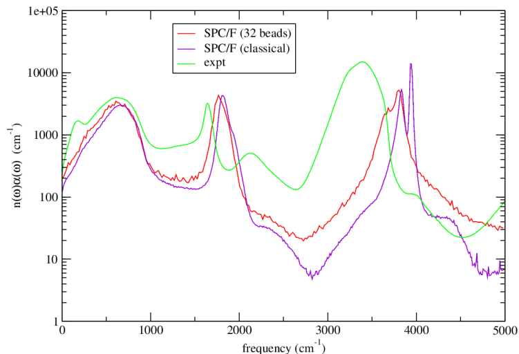
Figure 11.8: Infrared spectra for SPC/F at 300 K. Experimental data from Bertie & Lan, 1996.[15] PA-CMD was used, with normal mode frequencies scaled to 5000 \text{cm}^{-1} .
