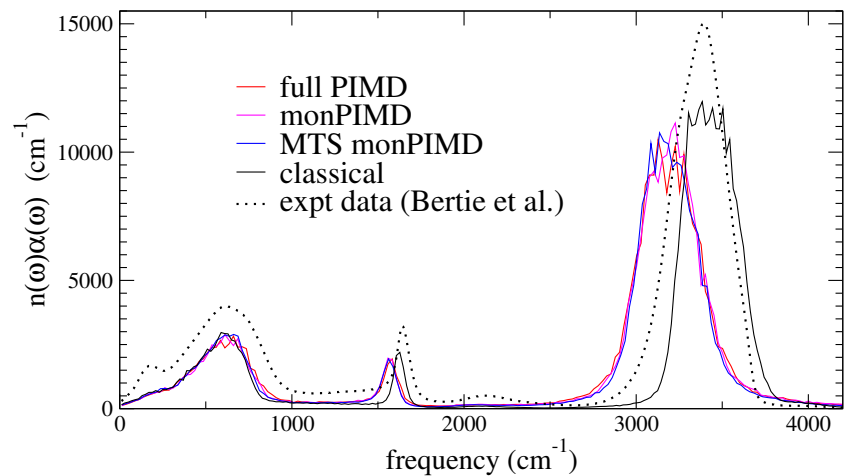
Figure 12.4: Validation with TTM3F: infrared spectra for the three PIMD methods compared to the classical spectra and experimental data at 300 K. [15]
