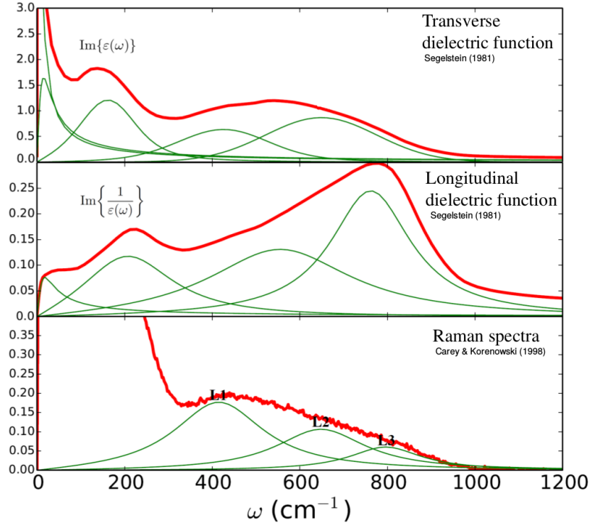
Figure 10.2: A figure highlighting the discrepancy in peak assignment. Dielectric functions derived from a compilation of experimental data by Segelstein,[12] with fits by D. C. Elton, while the Raman data comes from (Carey, 1998).[13] The Raman peaks are not fit but merely placed at the positions reported from Carey’s fit.
