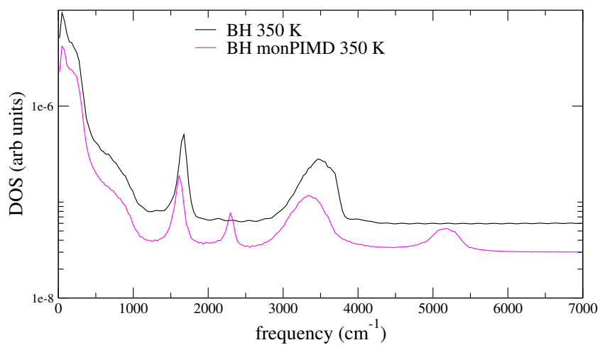
Figure 12.9: Density of states (eqn. 12.27) for 64 molecules with conventional MD, compared with the monomer PIMD method (32 beads).
