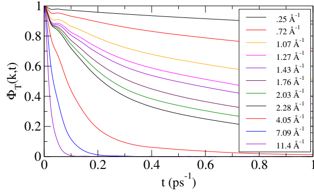
Figure 10.5: Transverse polarization relaxation functions for TIP4P/ \varepsilon . The librational mode at small k is heavily damped.
