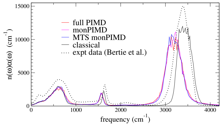
Figure 12.4: Validation with TTM3F: infrared spectra for the three PIMD methods compared to the classical spectra and experimental data at 300 K. [15]
