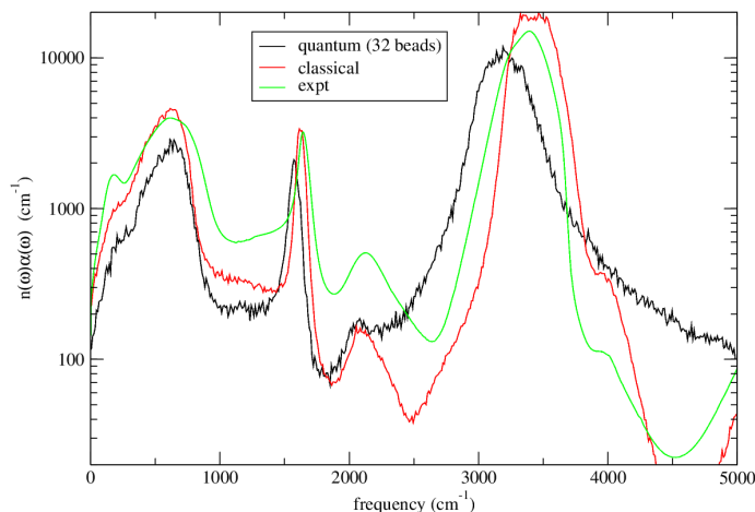
Figure 11.7: Infrared spectra for TTM3F at 300 K, plotted on a log scale to show detail. Experimental data from Bertie & Lan, 1996. [15] PA-CMD was used, with normal mode frequencies scaled to 5000 \text{ cm}^{-1} .
