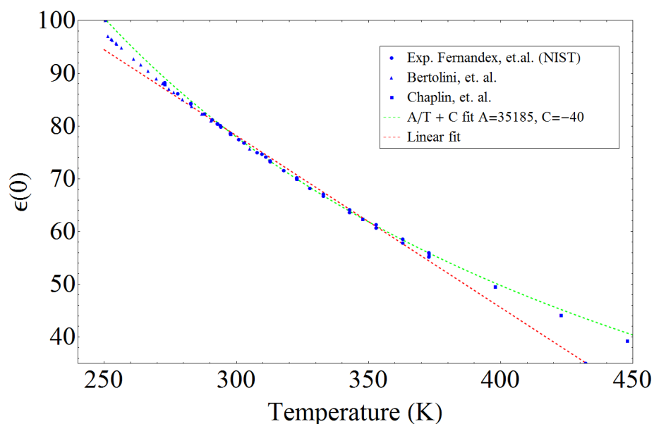
Figure 2.1: Experimental data on \varepsilon(0) taken from Fernandez et al., [1] Bertolini, et al., [2] and Chaplin et al. [3] Although a \varepsilon(0)(T) is roughly linear in the range 273 - 373 K, the overall behaviour is better described by A/T + C . The data above 373 K is taken along the liquid-vapor coexistence curve with increased pressure.
